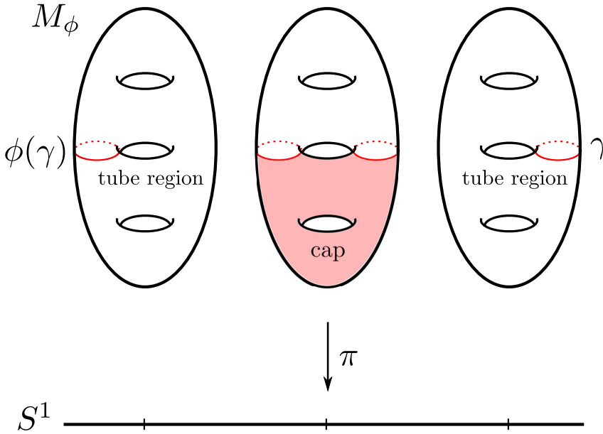
Figure 1: A tube surface
