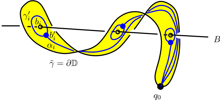
FIGURE 2.1. Kernel
